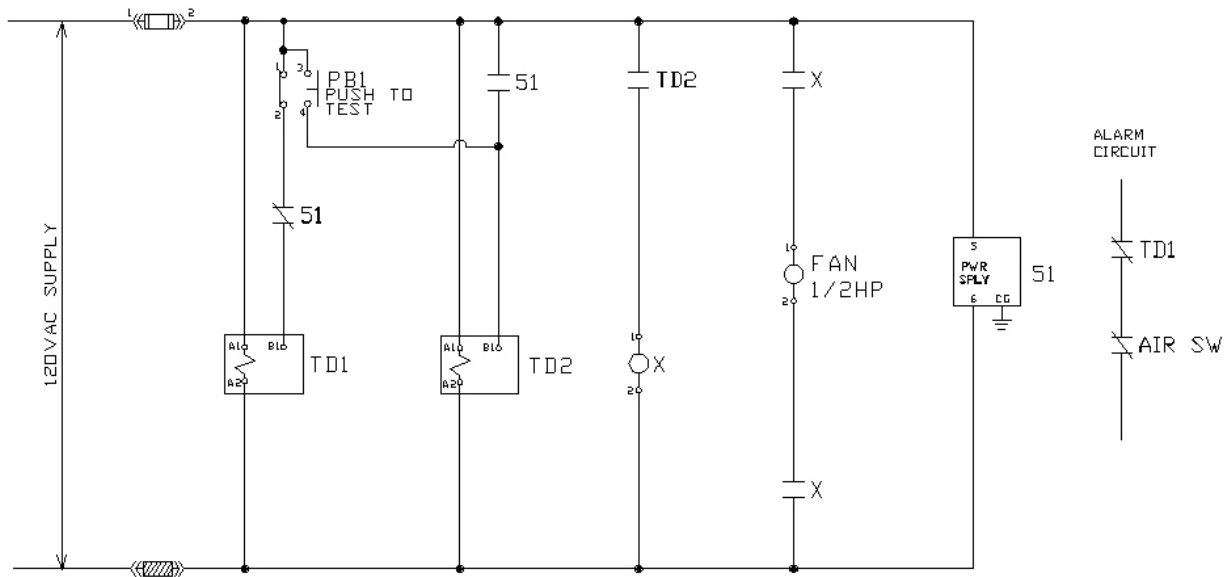
Typical Fan-Cooling Control Circuit Schematic Diagram
