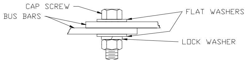
Figure 1: Anatomy of a bolted bus bar joint
