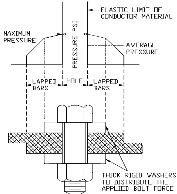
Figure 2: Distribution of forces in a bolted bus bar joint
